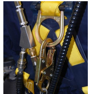
Figure 5: "D" ring connection
